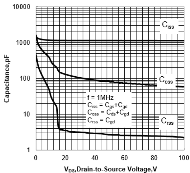
Figure 10 Capacitance Characteristics
